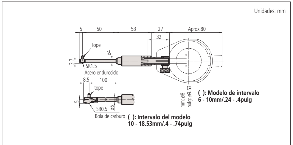
511-209/511-214 Tope
